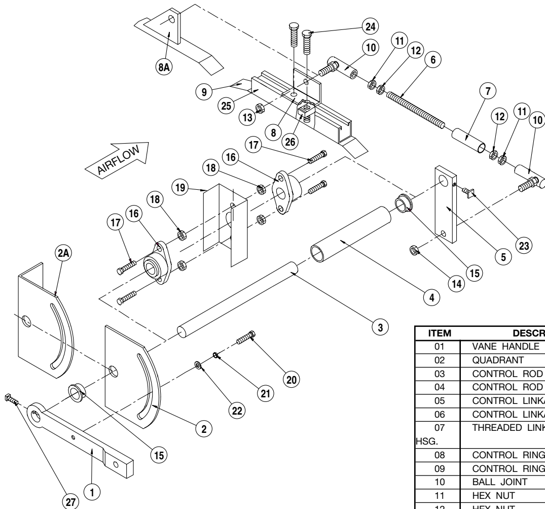
Figure 2. Nested Inlet Vane Control System for SWSI BC, BAF, BCS Fans
