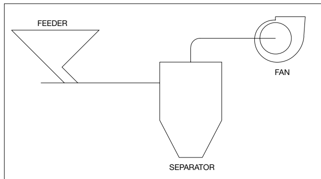
Figure 2. Negative Pressure – Dilute Phase Layout
